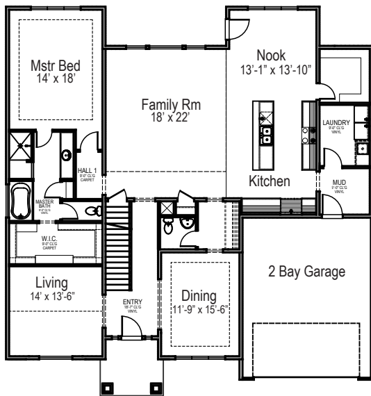
Main Level Floor Plan
